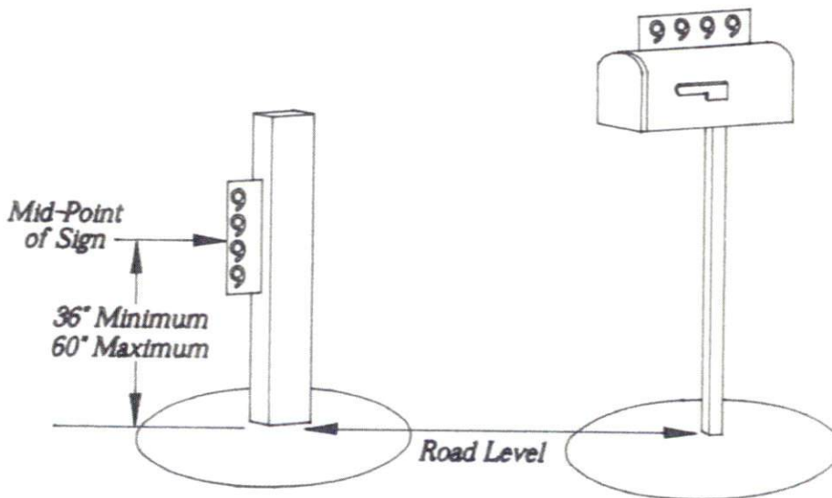
Free-Standing Post
